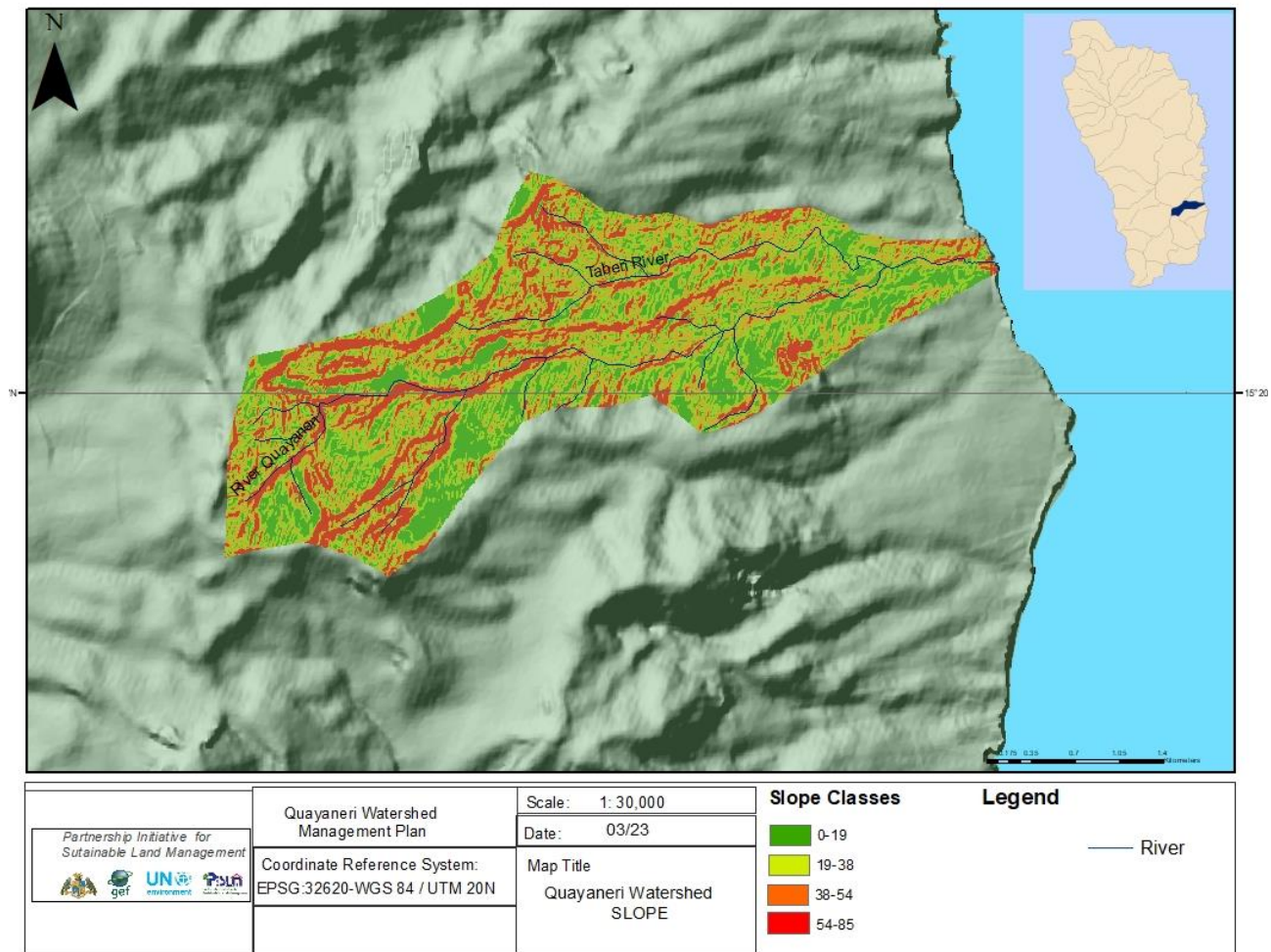
Figure 3: Slope characterization of the Quyaneri Watershed
