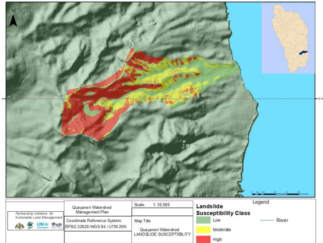
Figure 12: Landslide susceptibility within the BW
